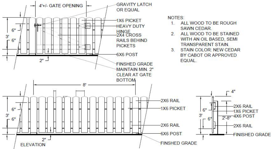
Figure 2. Fence and Gate Specification
